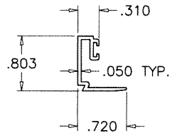
3 GLAZING BEAD (5/16" GLASS)
