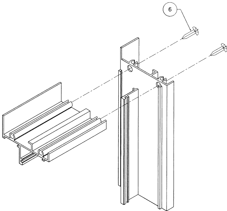
FRAME CORNER
