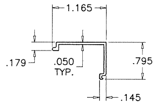
2 FRAME COVER
