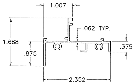
1 WINDOW FRAME
