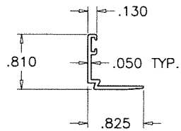
3A GLAZING BEAD (7/16" GLASS)
